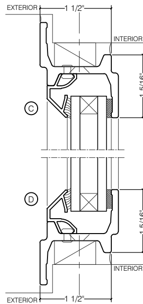
CASEMENT/FIXED/CASEMENT
