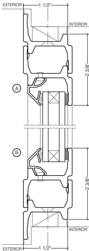
CASEMENT/FIXED
