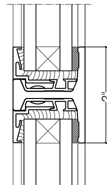
1" GLASS MAX.
