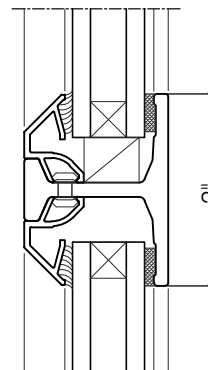
3/4" GLASS
