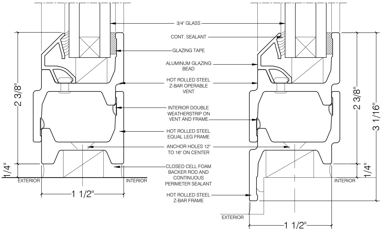
EQUAL LEG FRAME WITH OPERABLE VENT
