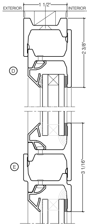
HOPPER OVER FIXED
