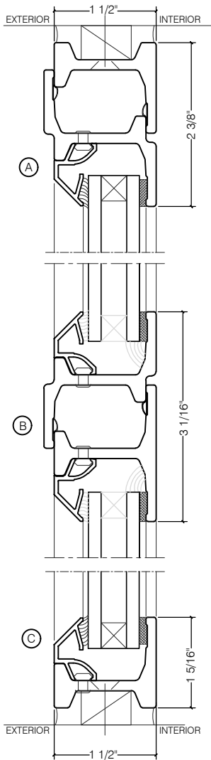
AWNING OVER FIXED
