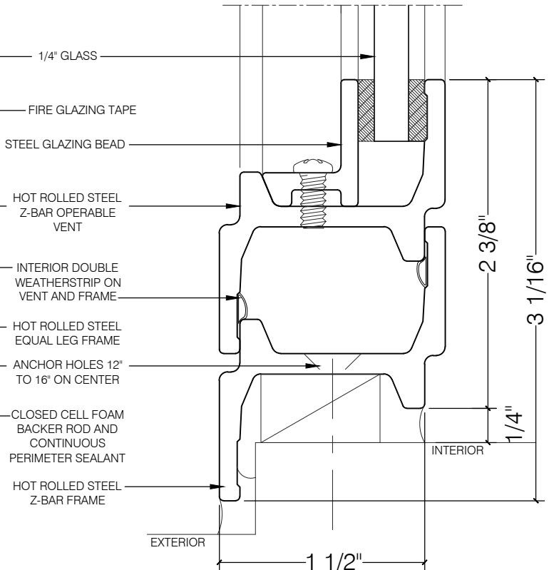
Z-BAR FRAME WITH OPERABLE VENT
