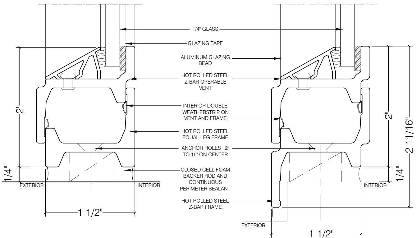
EQUAL LEG FRAME WITH OPERABLE VENT
