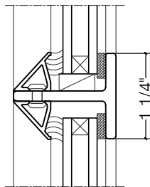
1/2" GLASS
