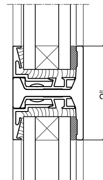
1" GLASS MAX.
