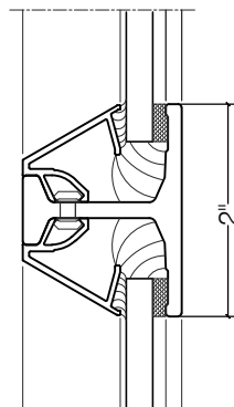
1/4" GLASS
