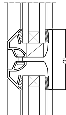
3/4" GLASS
