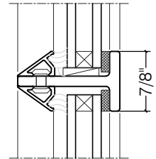
1/2" GLASS
