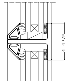
5/8" GLASS
