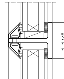
3/4" GLASS MAX.
