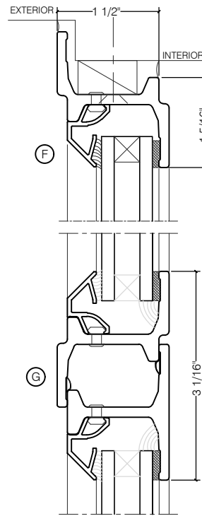
FIXED WITH HOPPER
