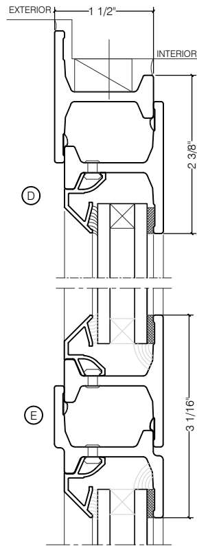
HOPPER OVER FIXED
