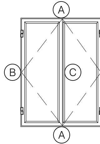
IN-SWING DOUBLE CASEMENT
