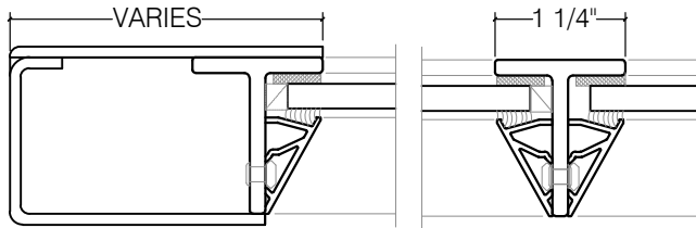
SLOPED BEAD FOR 1/4" GLASS
