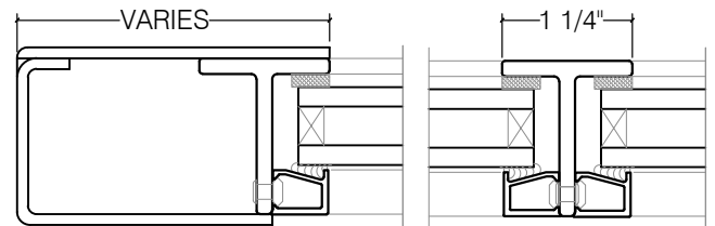
SQUARE BEAD FOR 3/4" GLASS
