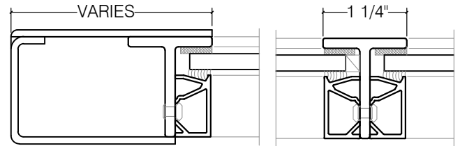
SQUARE BEAD FOR 1/4" GLASS
