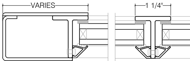
SLOPED BEAD FOR 3/4" GLASS
