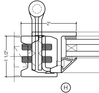
SWING IN 5/8" GLASS
